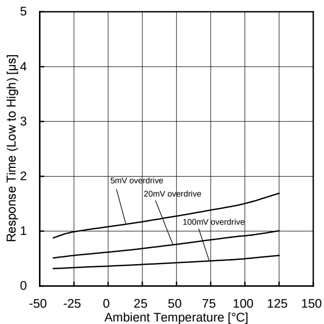
Figure 85. Response Time (Low to High) vs Ambient Temperature ( V_{CC}=5V , V_{RL}=5V , R_L=5.1k\Omega )
