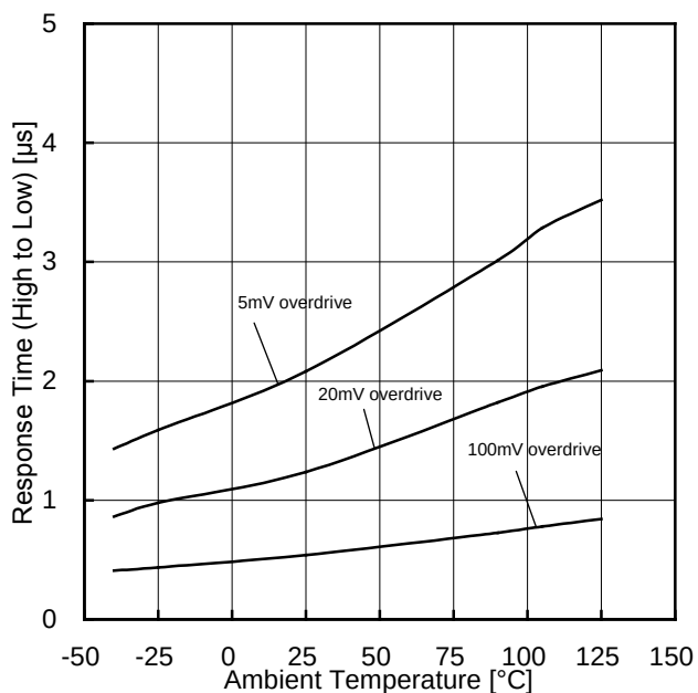
Figure 87. Response Time (High to Low) vs Ambient Temperature ( V_{CC}=5V , V_{RL}=5V , R_L=5.1k\Omega )
