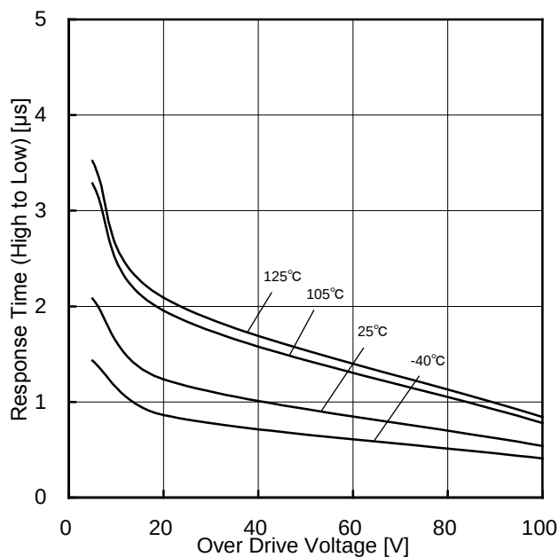
Figure 86. Response Time (High to Low) vs Over Drive Voltage ( V_{CC}=5V , V_{RL}=5V , R_L=5.1k\Omega )
