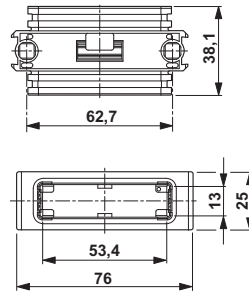
D-SUB coupling
