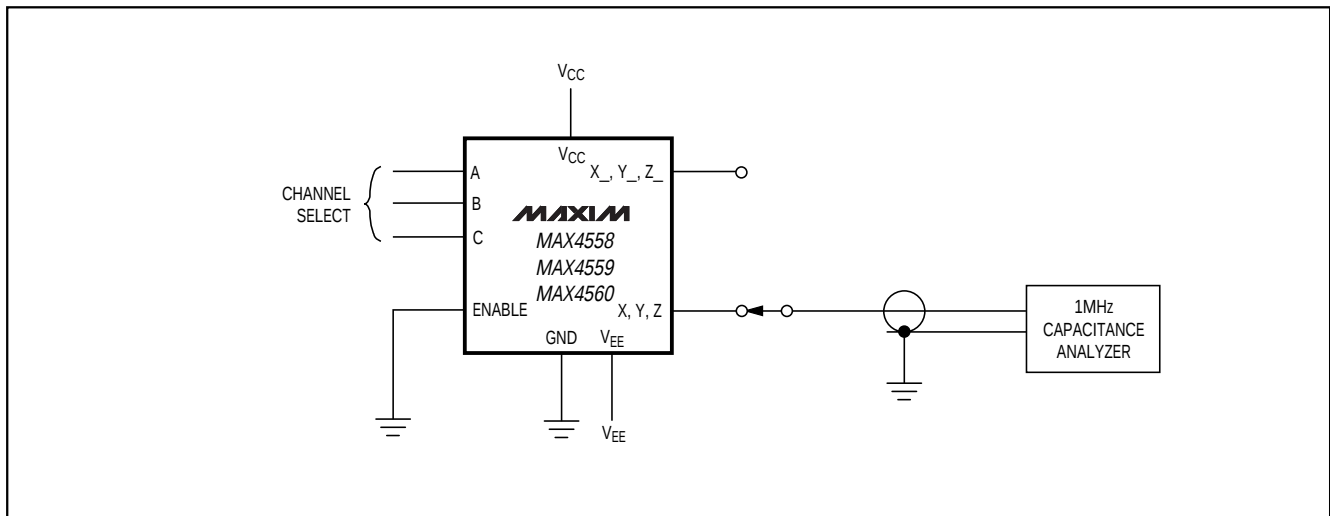
Figure 5. Channel Off/On-Capacitance
