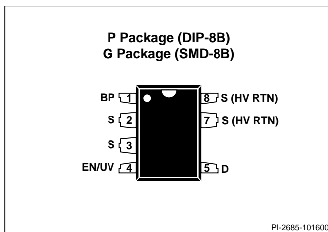
Figure 3. Pin Configuration.
