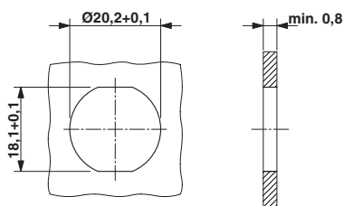
Dimensional drawing
