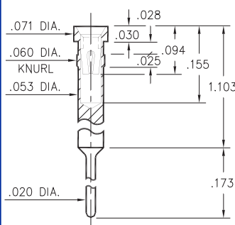
3018-0-15-XX-30-XX-04-0 Press-fit in .057 mounting hole
