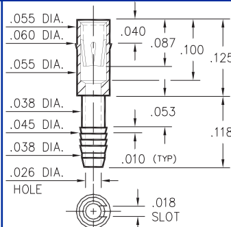
4310-0-31-XX-43-XX-04-0 Compliant press-fit in .040±.003 plated hole. For .090→.130 thick board.
