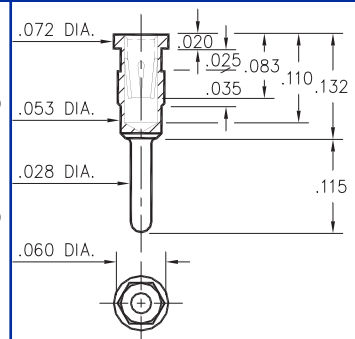
5960-0-15-XX-43-XX-04-0 Hex press-fit in .057 plated thru hole
