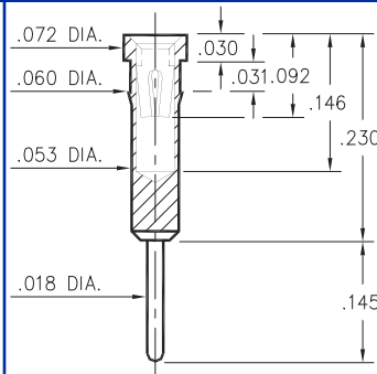
4001-0-15-XX-43-XX-04-0 Press-fit in .057 mounting hole
