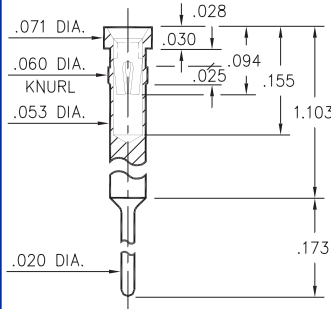
3018-0-15-XX-30-XX-04-0 Press-fit in .057 mounting hole
