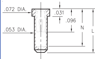
XXXX-0-15-XX-30-XX-10-0 Solder mount in .055 min. mounting hole Also available on 16mm wide carrier tape: 1,700 parts per 13" reel. Order as: XXXX-0-57-XX-30-XX-10-0
