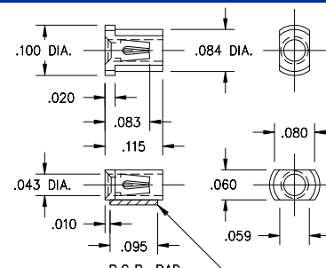
3907-0-18-XX-30-XX-10-0 Surface mount Also available on 12mm wide carrier tape: 4,000 parts per 13" reel. Order as: 3907-0-58-XX-30-XX-10-0
