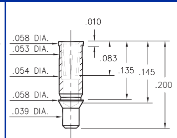
1385-0-15-XX-43-XX-10-0 Surface mount
