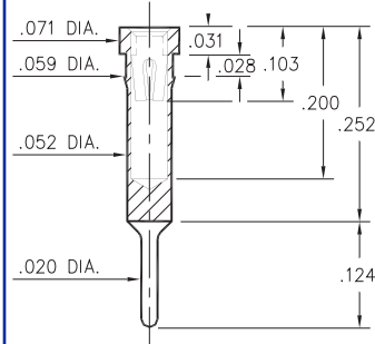
8852-0-15-XX-30-XX-04-0 Press-fit in .056 mounting hole
