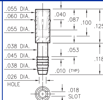
4310-0-31-XX-43-XX-04-0 Compliant press-fit in .040±.003 plated hole. For .090→.130 thick board.
