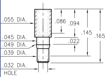
0385-0-15-XX-43-XX-10-0 Press-fit in .046 mounting hole
