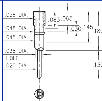
1782-0-15-XX-43-XX-04-0 Press-fit in .045 mounting hole
