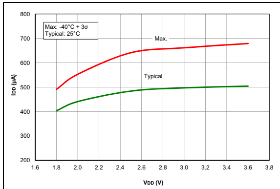
FIGURE 35-49: I_{DQ} , Comparator, NP Mode ( CxSP = 1 ), PIC16LF1717/8/9 Only.
