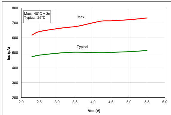
FIGURE 35-50: I_{DQ} , Comparator, NP Mode ( CxSP = 1 ), PIC16F1717/8/9 Only.
