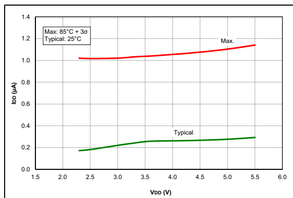
FIGURE 35-48: I_{D} , ADC Non-Converting, PIC16F1717/8/9 Only.
