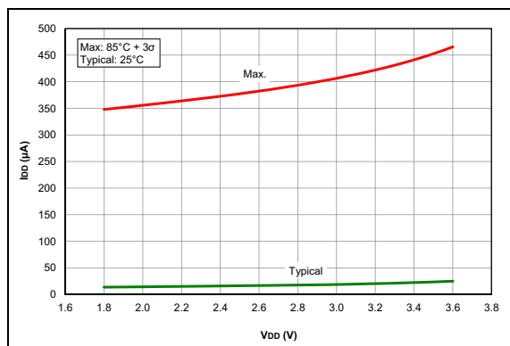
FIGURE 35-47: I_{D} , ADC Non-Converting, PIC16F1717/8/9 Only.
