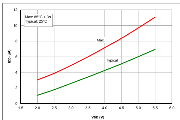
FIGURE 35-44: I_{D} , Timer1 Oscillator, F_{OSC} = 32\text{ kHz} , PIC16F1717/8/9 Only.
