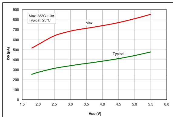
FIGURE 35-46: I_{D} , Op Amp, High GBWP Mode ( OPAxSP = 1 ), PIC16F1717/8/9 Only.
