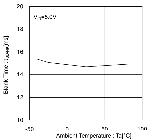
Figure 26. Blank Time vs Ambient Temperature
