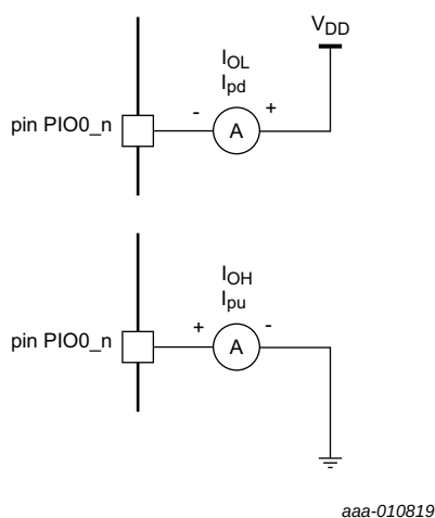
Fig 17. Pin input/output current measurement
