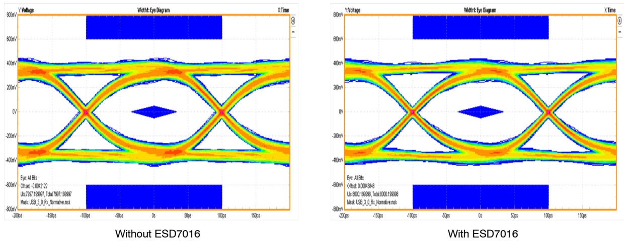
Figure 10. USB3.0 Eye Diagram with and without ESD7016, 5 Gb/s
