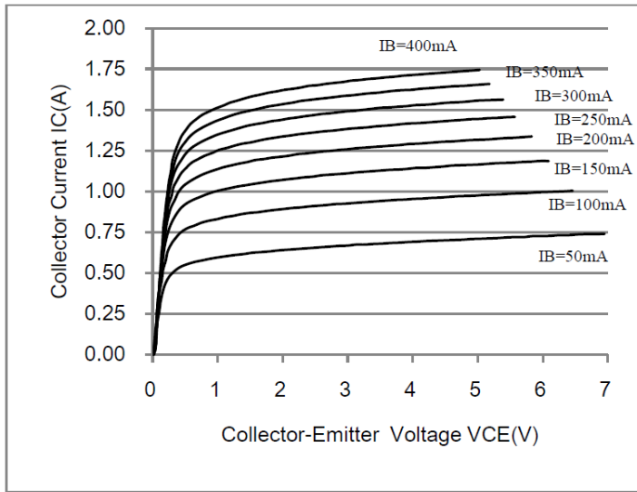
Static Characteristics
