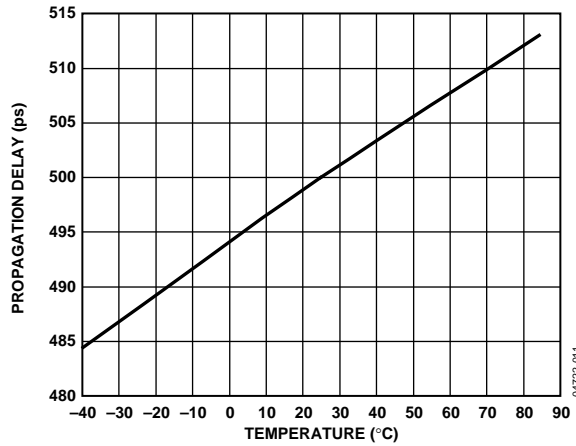
Figure 11. Propagation Delay vs. Temperature
