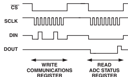
Figure 6. The Serial Interface Signals—Register Access
