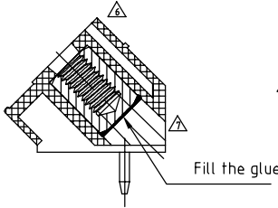
SECTION P-P
