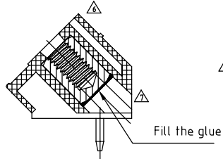
SECTION P-P
