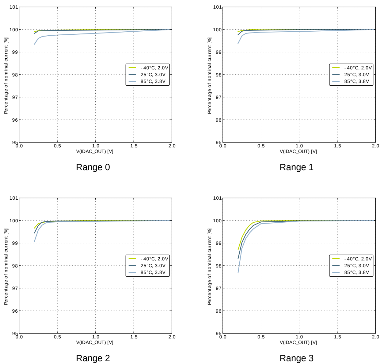
Figure 3.34. IDAC linearity
