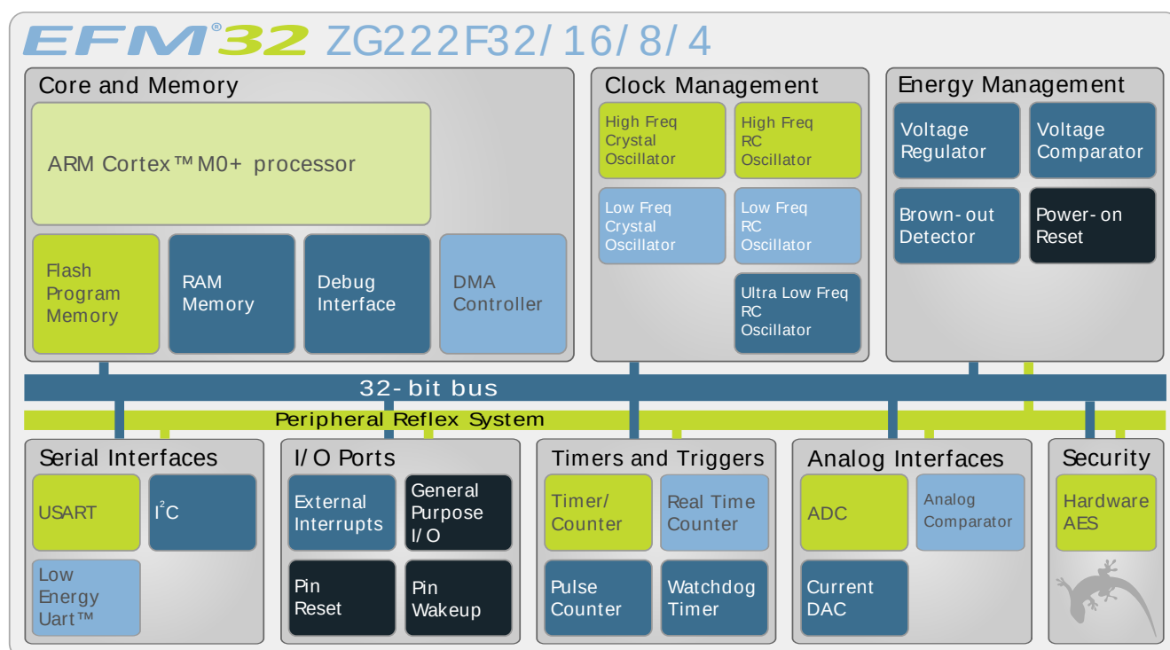
Figure 2.1. Block Diagram
