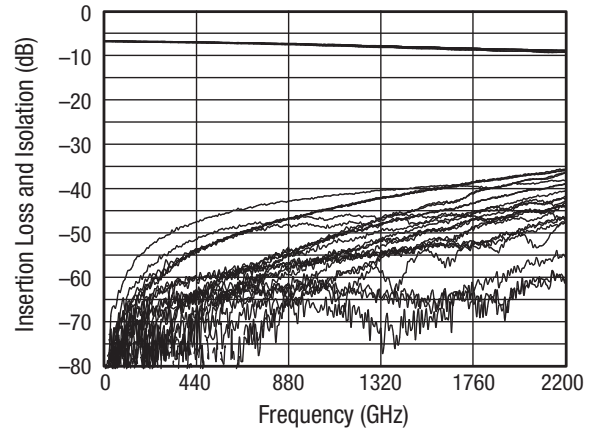
Figure 7. I4 to OUT1 and I4 to OUT2 Paths for States 0 to 15
