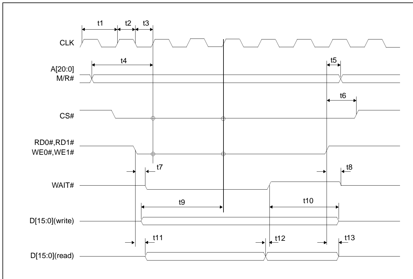
Figure 7-6: Generic Timing
