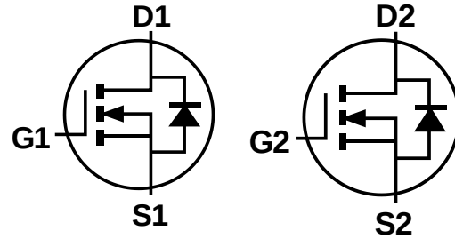
Internal Schematic
