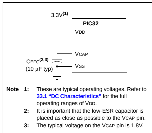
FIGURE 30-1: CONNECTIONS FOR THE ON-CHIP REGULATOR
