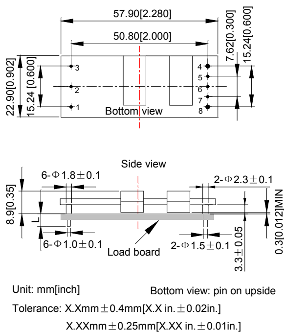
Figure 21 Mechanical diagram
