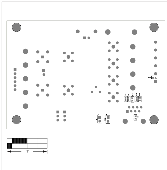
MAX22502E EV Kit—Bottom Silkscreen
