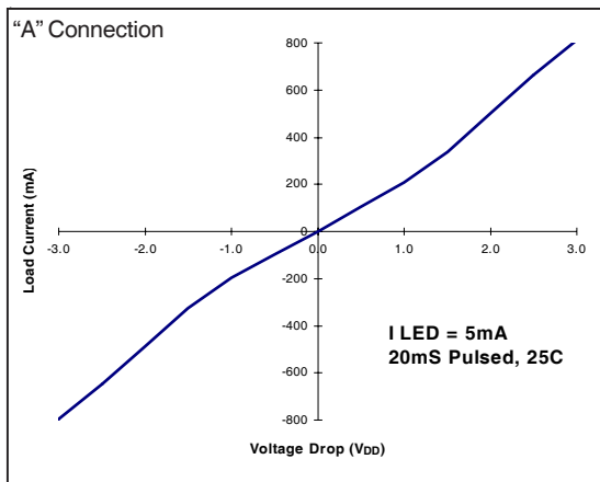
Figure 2. Typical On Characteristics
