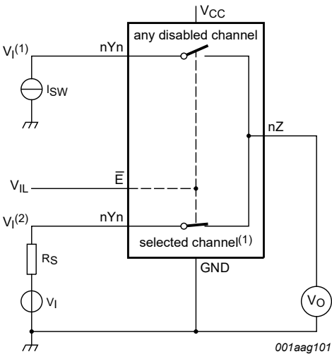
Fig. 9. Test circuit for injection current coupling
