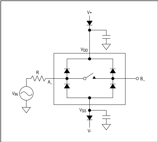
Figure 10. Beyond-the-Rail Application
