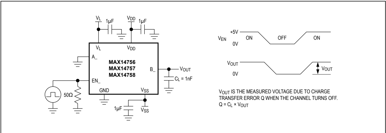
Figure 8. Charge Injection
