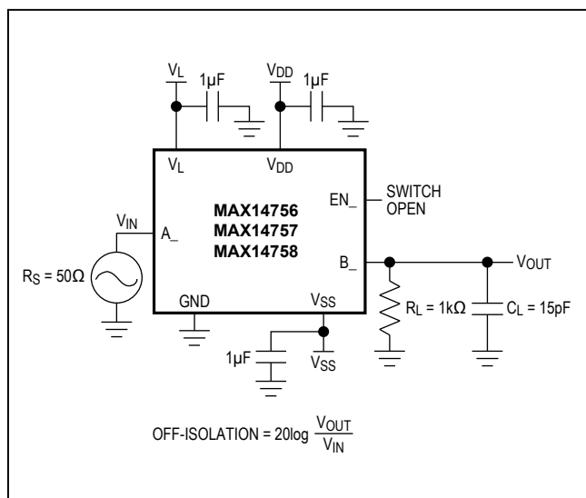
Figure 5. Off-Isolation
