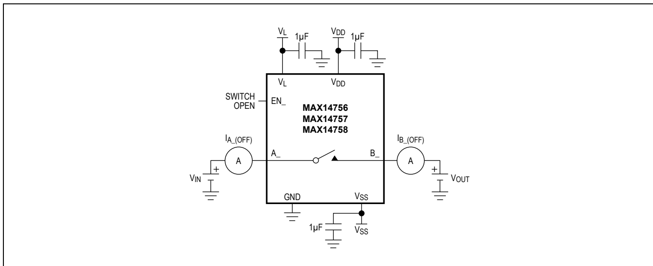
Figure 3. Off-Leakage Current
