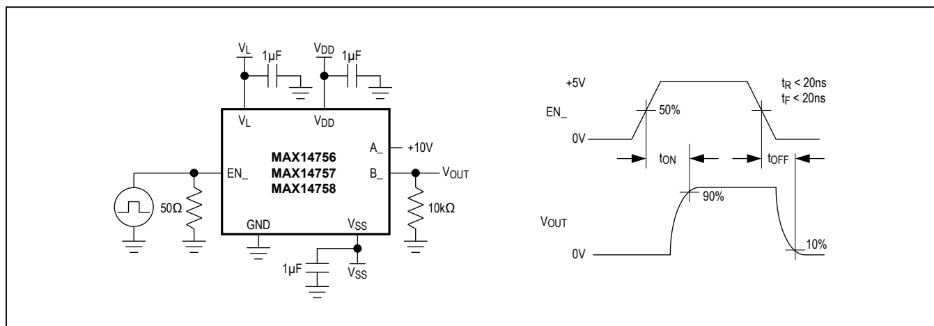
Figure 4. Enable Switching Time
