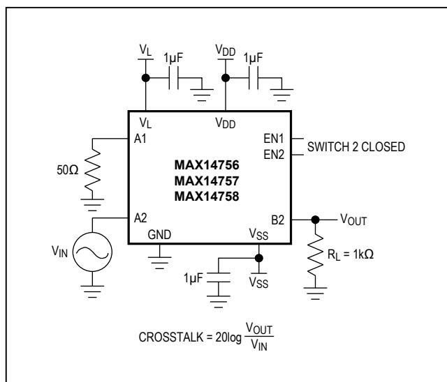
Figure 6. Crosstalk
