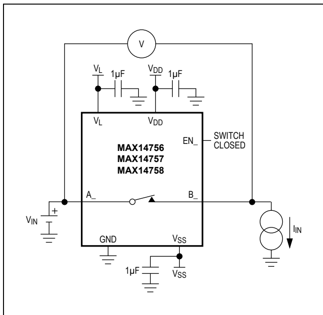
Figure 1. On-Resistance Measurement
