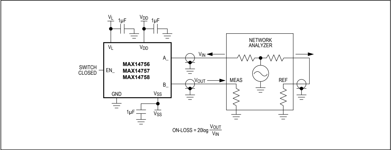
Figure 7. Frequency Response
