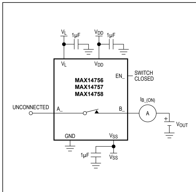
Figure 2. On-Leakage Current
