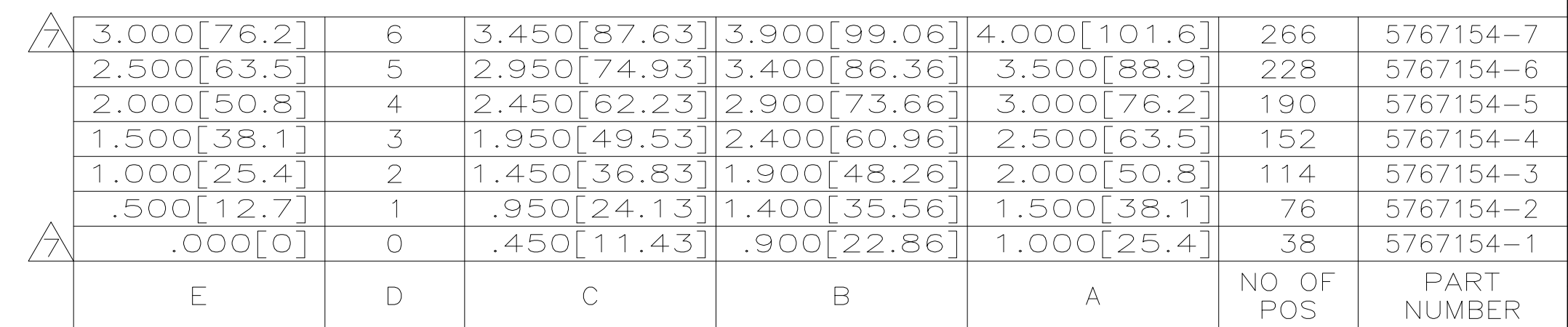
THIS DRAWING IS A CONTROLLED DOCUMENT. DWN. 26 OCT 04 A. FERNANDEZ Tyco Electronics Corporation Harrisburg, Pa 17105-3608 DIMENSIONS: INCHES TOLERANCES UNLESS OTHERWISE SPECIFIED: Tyco Electronics D. DIXON 26 OCT 04 NAME APPRO. D. DIXON 26 OCT 04 RECEPTACLE ASSEMBLY, .355[9.02] VERTICAL, .025[0.64] CENTER LINE, MICTOR PRODUCT SPEC 108-1422 APPLICATION SPEC 114-11004 SIZE CAGE CODE DRAWING NO WEIGHT A1 00779 C-5767154 CUSTOMER DRAWING RESTRICTED TO — MATERIAL FINISH SCALE 8:1 SHEET 1 OF 1 REV B 1 2
