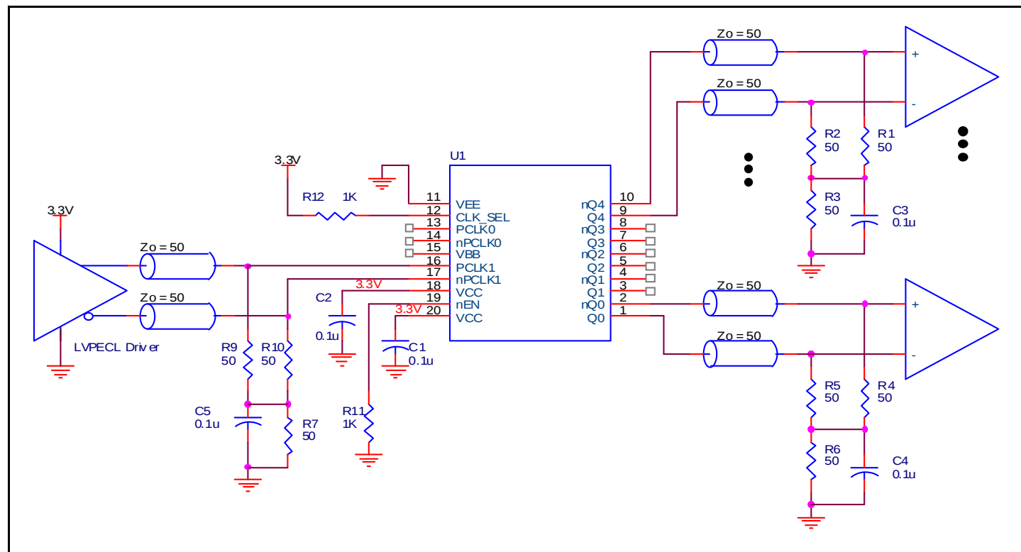
Figure 6. ICS853S014I Example LVPECL Clock Output Buffer Schematic
