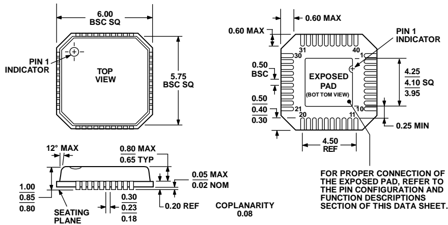
COMPLIANT TO JEDEC STANDARDS MO-220-VJJD-2 Figure 84. 40-Lead Lead Frame Chip Scale Package [LFCSP_VQ] 6 mm x 6 mm Body, Very Thin Quad (CP-40-1) Dimensions shown in millimeters
