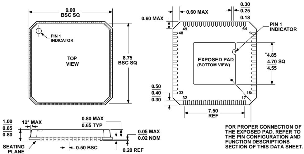
*COMPLIANT TO JEDEC STANDARDS MO-220-VMMD-4 EXCEPT FOR EXPOSED PAD DIMENSION Figure 85. 64-Lead Lead Frame Chip Scale Package [LFCSP_VQ] 9 mm x 9 mm Body, Very Thin Quad (CP-64-1) Dimensions shown in millimeters
