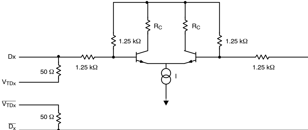
Figure 6. Input Structure
