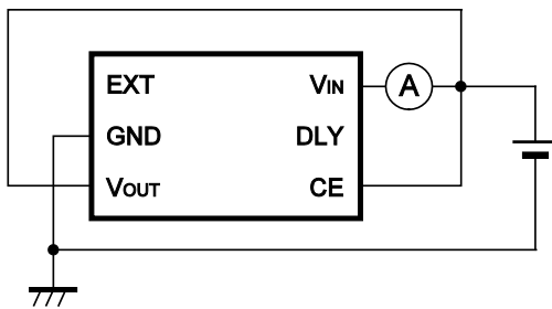
B) Supply Current 1
