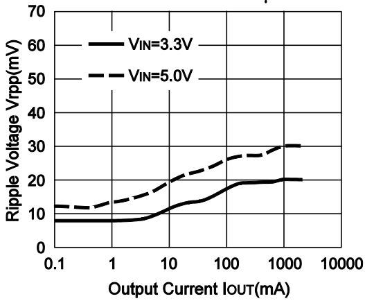
R1225N182A L=10μH
