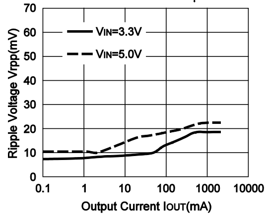
R1225N182B L=10μH
