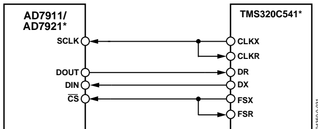
Figure 32. Interfacing to the TMS320C541
