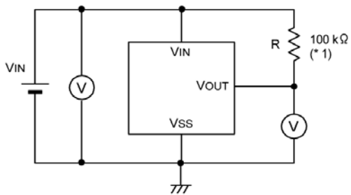
Circuit 1
