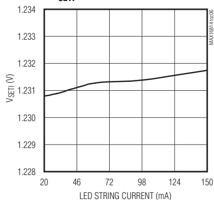
VSETI vs. PROGRAMMED CURRENT
