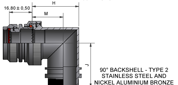
90° BACKSHELL - TYPE 2
