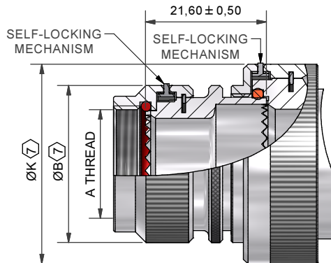
BACKSHELL - TYPE 2
