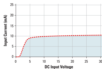
Input Current vs Input Voltage
