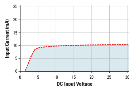
Input Current vs Input Voltage
