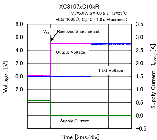
(32) Short-Circuit Transient Response
