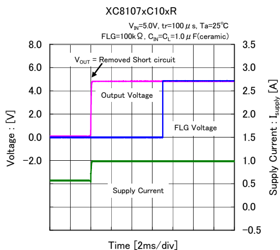
(30) Short-Circuit Transient Response
