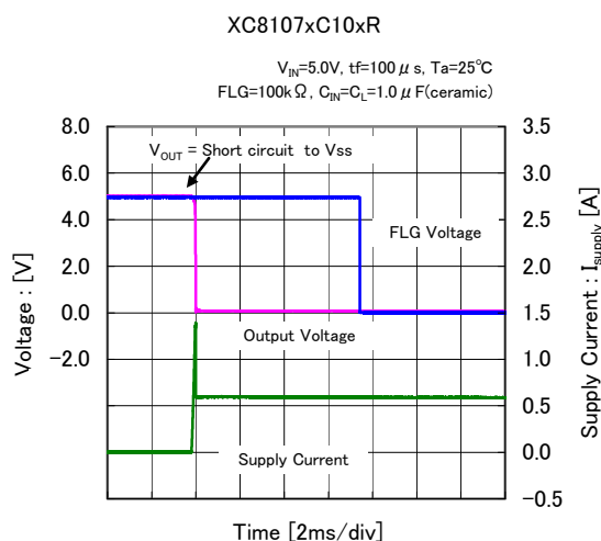
(31) Short-Circuit Transient Response
