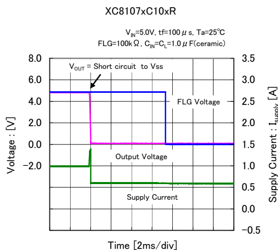
(29) Short-Circuit Transient Response
