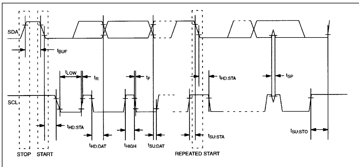
Figure 3. TIMING DIAGRAM
