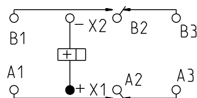
TERMINAL VIEW
