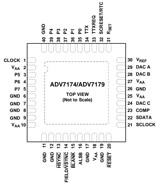
Figure 5. Pin Configurations
