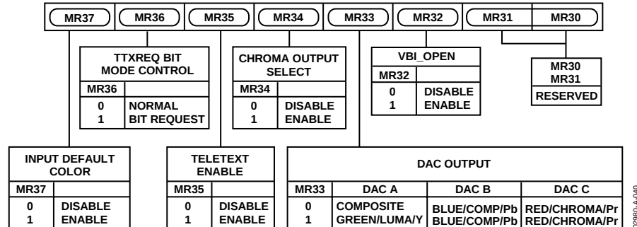
Figure 41. Mode Register 3
