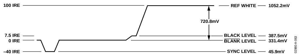
Figure 64. NTSC RGB Video Levels
