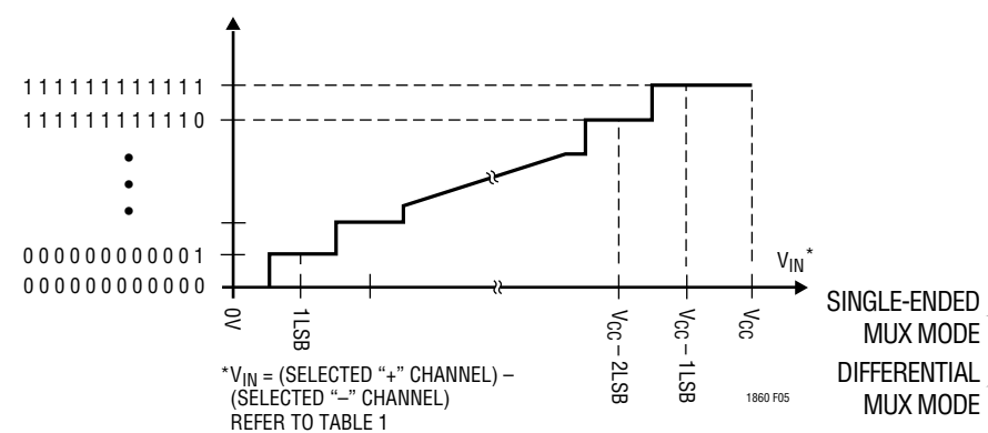
Figure 5. LTC1861 Transfer Curve
