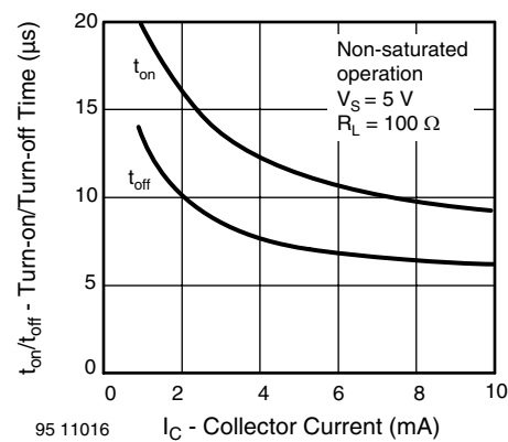
Fig. 17 - Turn-on/off Time vs. Collector Current
