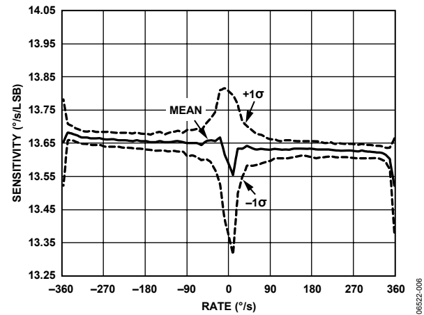
Figure 20. Gyroscope Linearity
