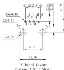
PC Board Layout Component Side Show
