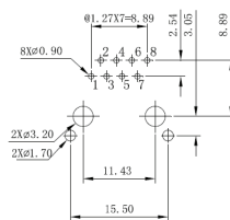
PC Board Layout Component Side Shown
