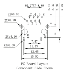
PC Board Layout Component Side Shows
